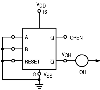
Figure 1. Output Source Current Test Circuit
