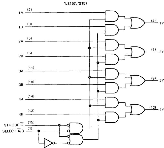
logic diagrams (positive logic)
