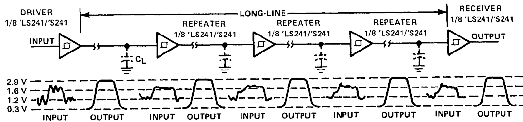
'LS241, 'S241 USED AS REPEATER/LEVEL RESTORER
