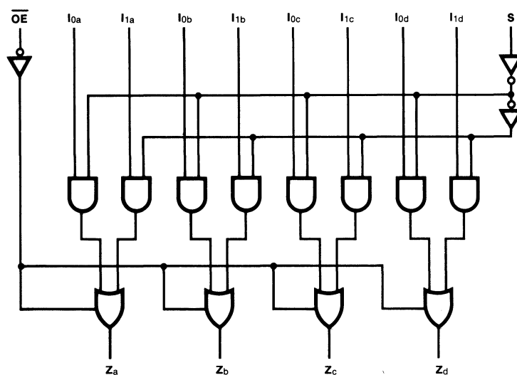
LOGIC DIAGRAM
