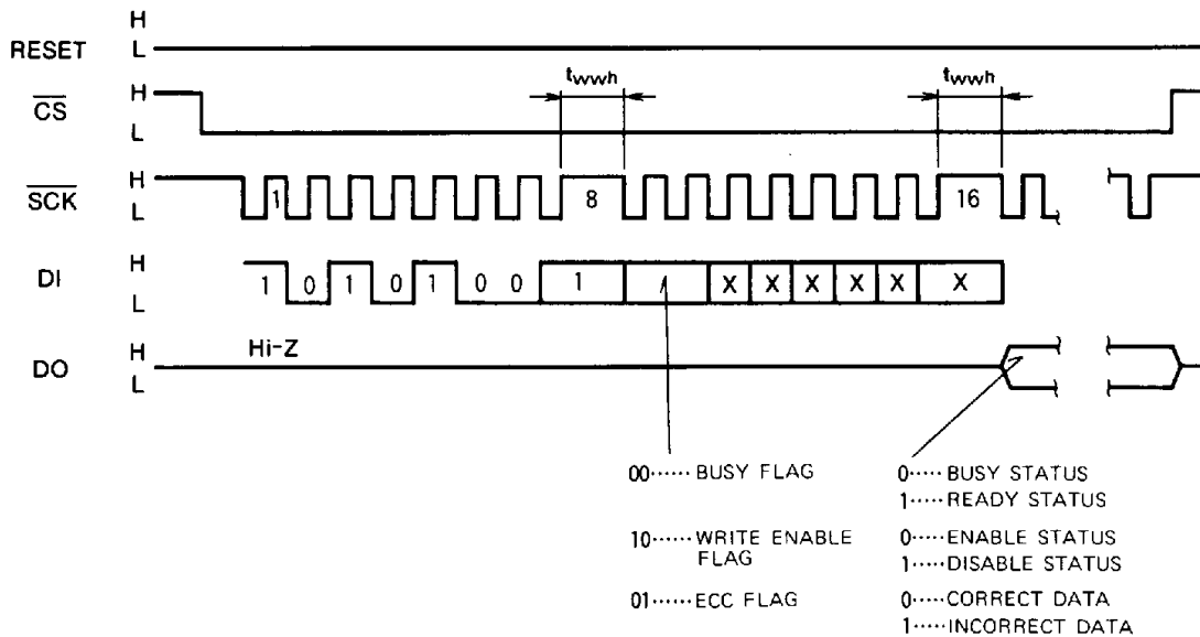
Fig. 3 Sequence at status output mode
