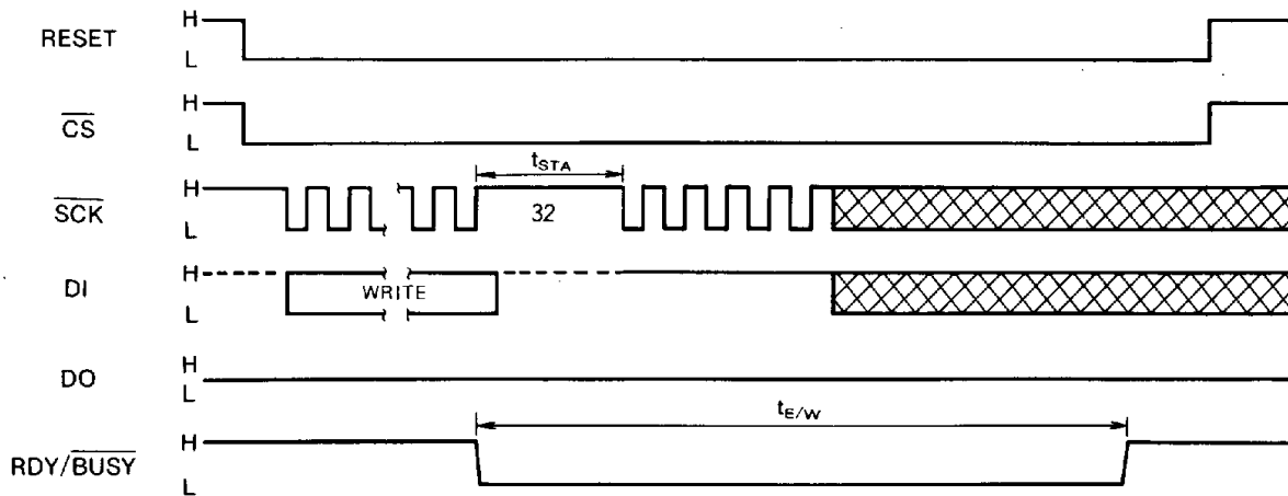
Fig. 10 Sequence of write operation
