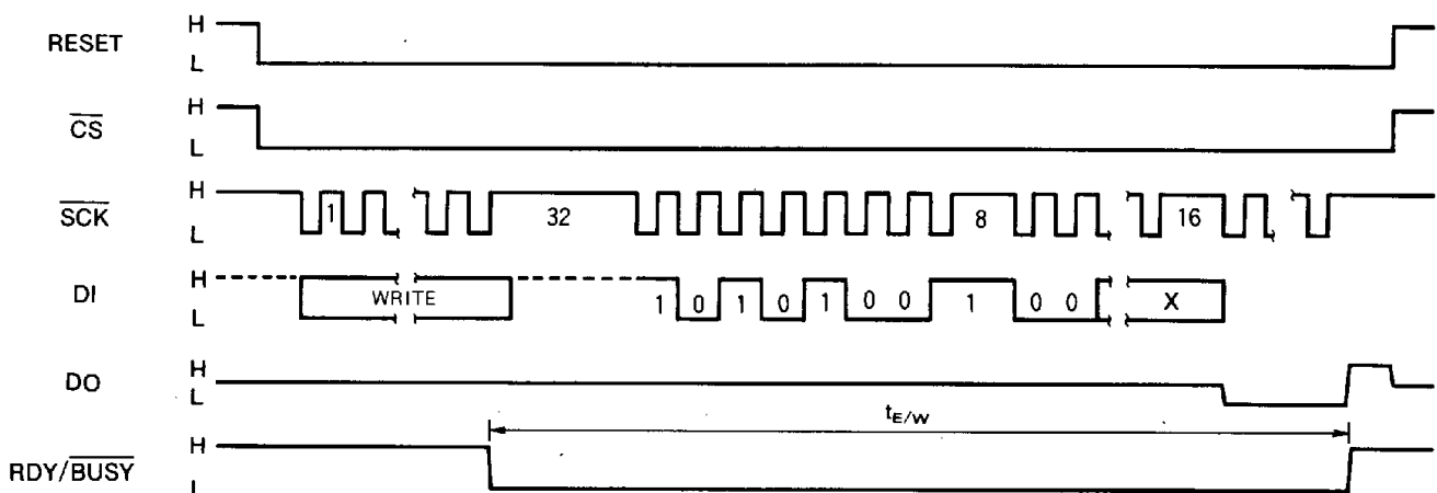
Fig. 9 Sequence of status output during write operation
