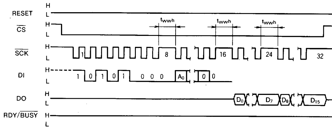
Fig. 4 Sequence at read mode
