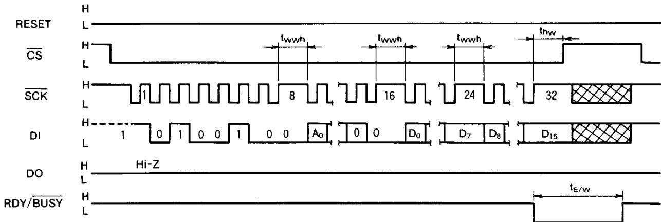
Fig. 6 Sequence at write mode
