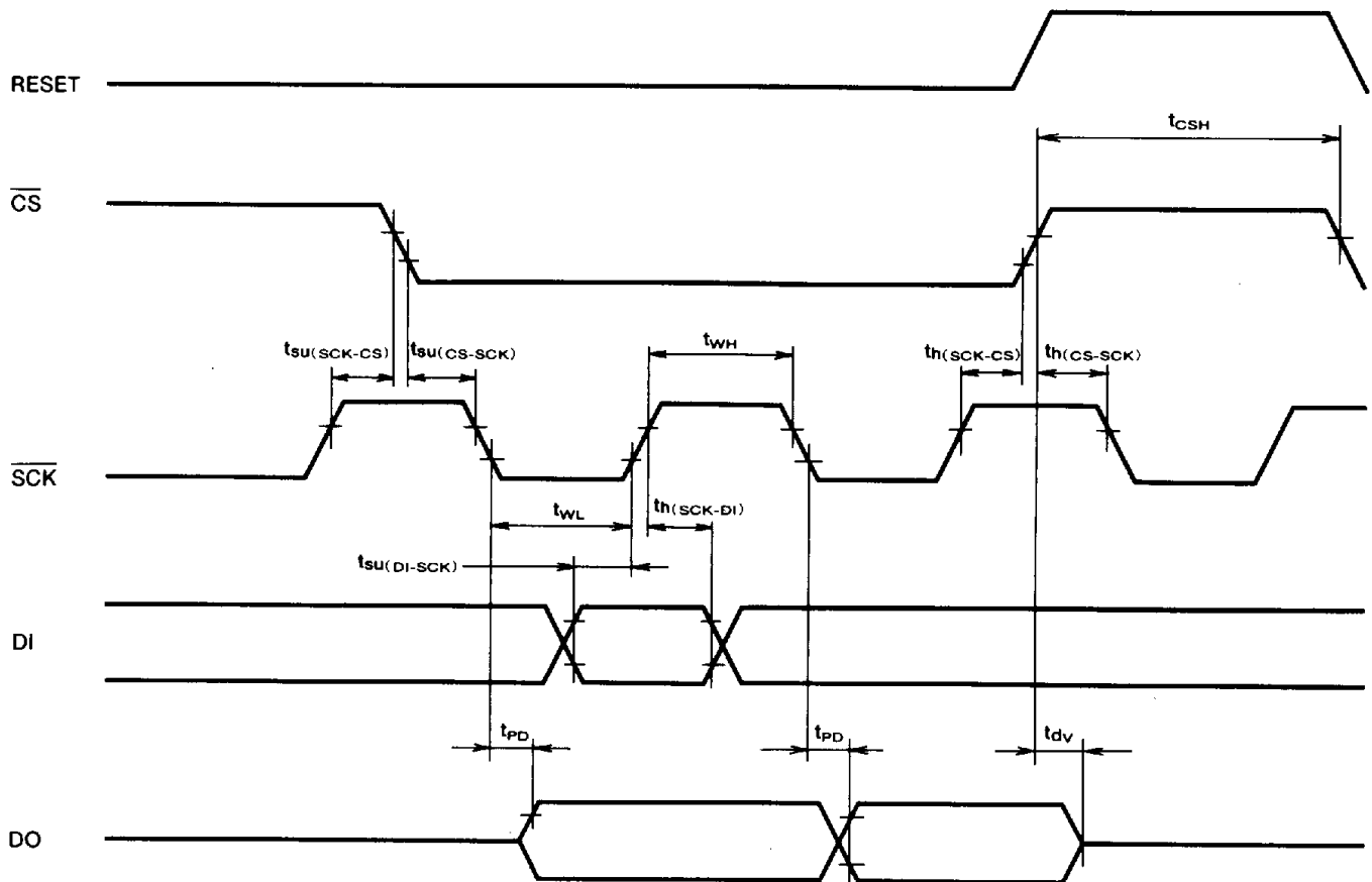
Fig. 1 Synchronizing timing
