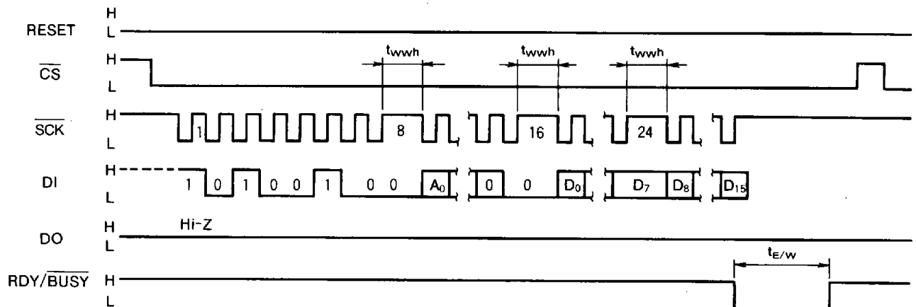
Fig. 5 Sequence at write mode
