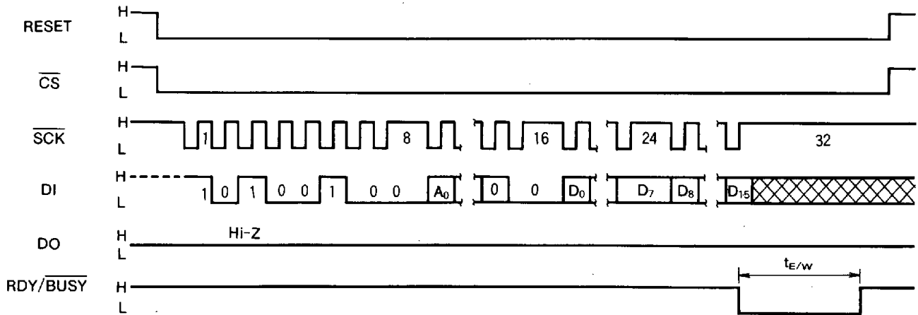
Fig. 8 Sequence of write operation
