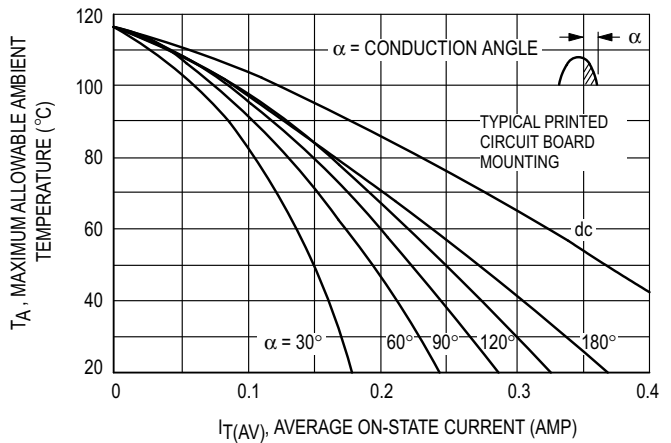
FIGURE 2 – MCR100-7, MCR100-8 CURRENT DERATING (REFERENCE: AMBIENT TEMPERATURE)
