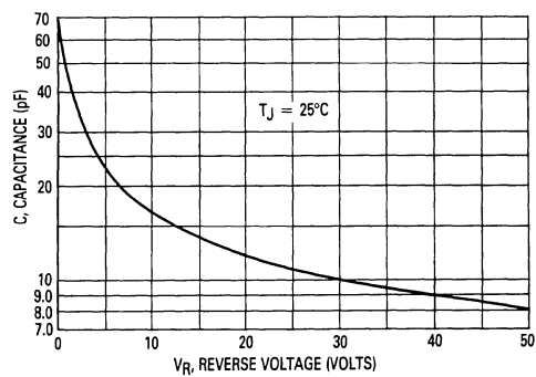
FIGURE 15 — TYPICAL CAPACITANCE
