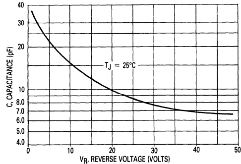
FIGURE 10 — TYPICAL CAPACITANCE
