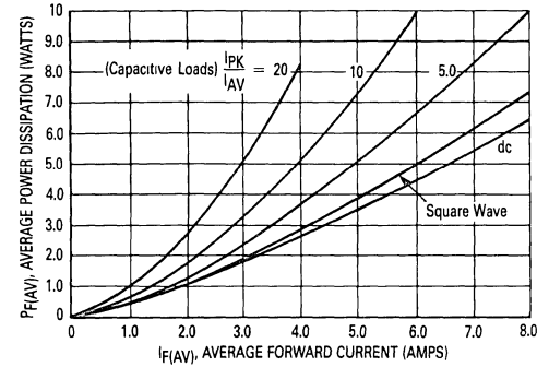
FIGURE 4 — POWER DISSIPATION
