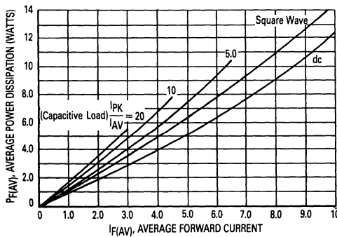
FIGURE 9 — POWER DISSIPATION
